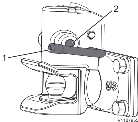
Trekhaakblad
